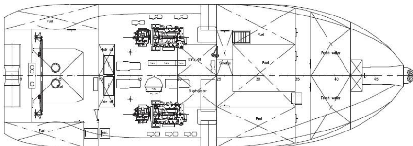
BELOW MAINDECK
