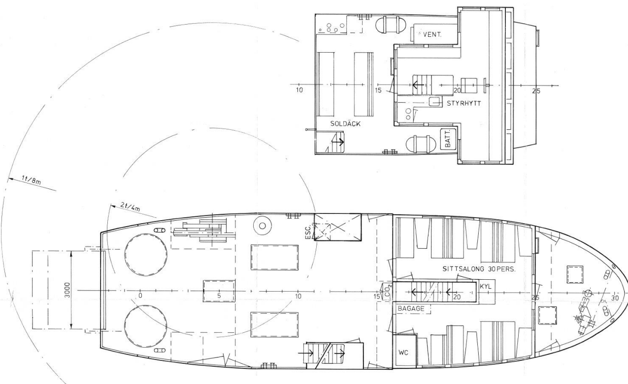
MAIN DECK
